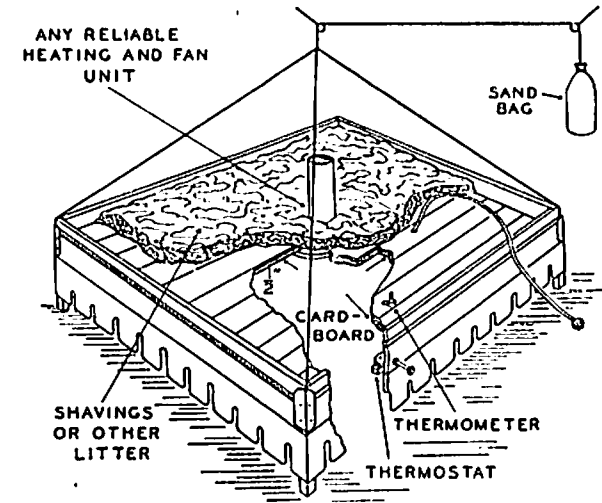
FIGURE 2. A HOMEMADE ELECTRIC BROODER FOR 300 OR 400 CHICKS.
