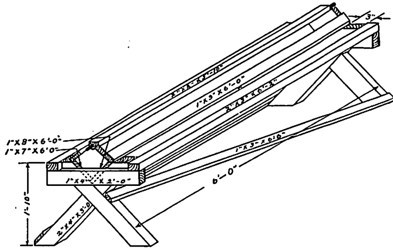
FIGURE 7. MASH HOPPERS FOR LAYERS—V-SHAPED TYPE.
