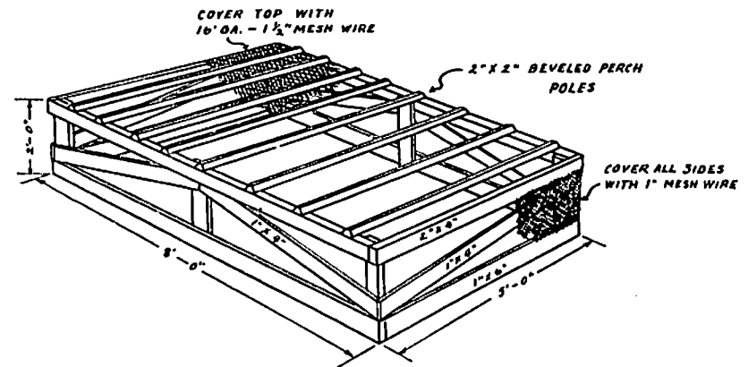
FIGURE 11. A PRACTICAL AND EASILY CONSTRUCTED ROOSTING RACK.
