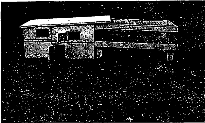
FIGURE 1. A HOMEMADE LAMP BROODER FOR 50-75 CHICKS. (FUEL USED—OIL OR ELECTRICITY)
