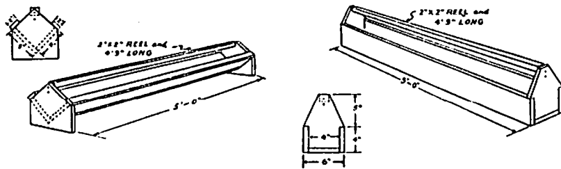
FIGURES 4A AND 4B. CHICK FEEDERS—INTERMEDIATE SIZE (FOR USE BY CHICKS 2 TO 7 WEEKS OF AGE)
